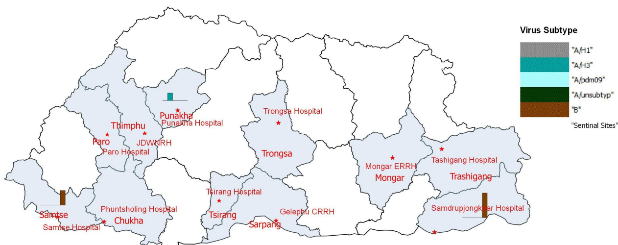
Figure 6: Influenza subtype virus by sentinel sites for week 44 (2014).
