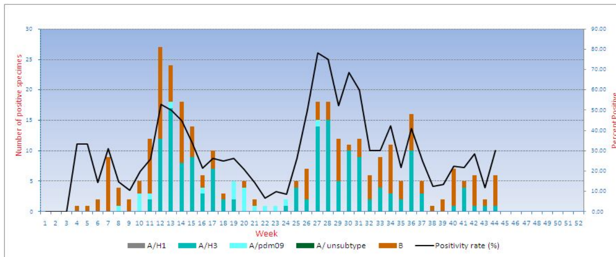
Figure 5: Trend of influenza virus subtype by week, for the week 44, 2014
