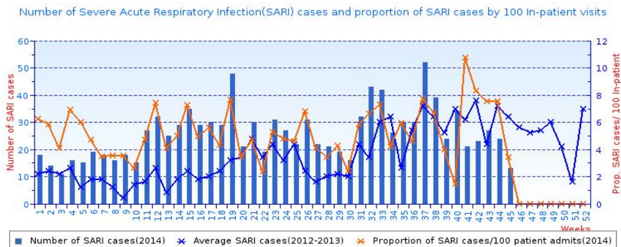
Figure 3: Average number of SARI cases reported for 45 week and previous weeks. (Data source: Online weekly reporting from sentinel sites).
