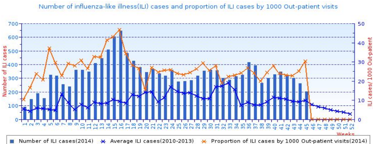
Figure 1: Average number of ILI cases reported for 45 week and previous weeks. (Data source: Online weekly reporting from sentinel sites.
