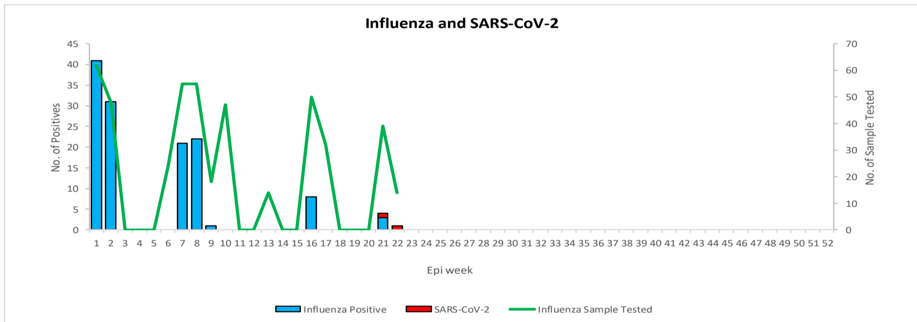
Figure 2: Weekly Influenza and SARS-CoV-2 detected from Flu sentinel sites (Source: RCDC)
