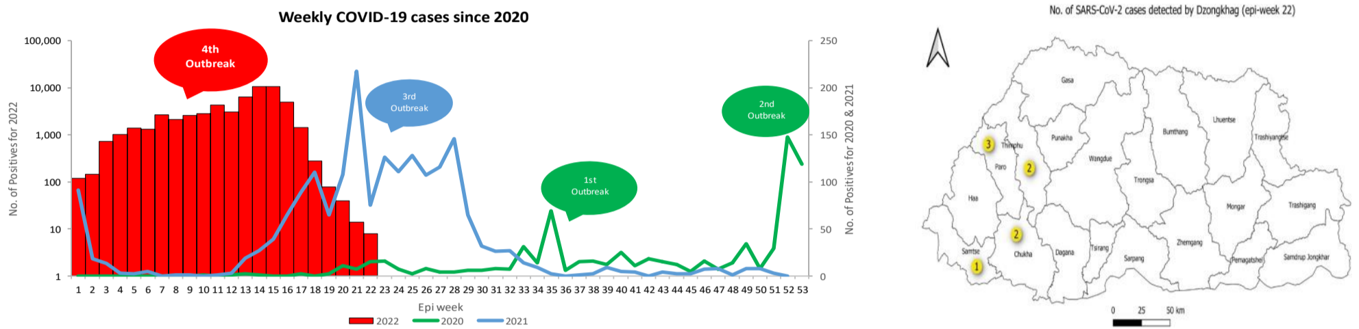
Figure 1: Weekly COVID-19 (SARS-CoV-2) detected from all across the country (Source: Ministry of Health dashboard)
